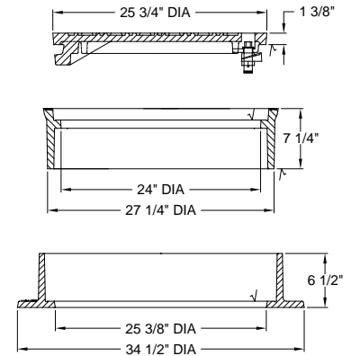
1208 adjustable frame and 1203A2 cover with optional cam lock illustrated
